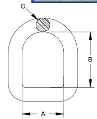
D-Ring with Clip (D-Ring and D-Ring Clip sold separately)
