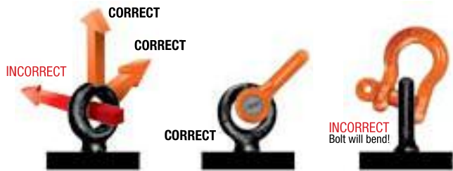
Shoulder Eye Bolt Working Load Limit Reductions based on Angle to Horizontal
