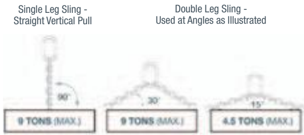
Working load limits for 5/8 inch alloy steel chain slings, (single and double leg configurations.)
